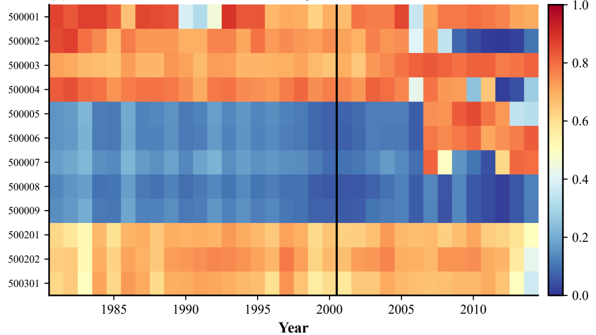
(b) Annual fraction of zero-rainfall days
