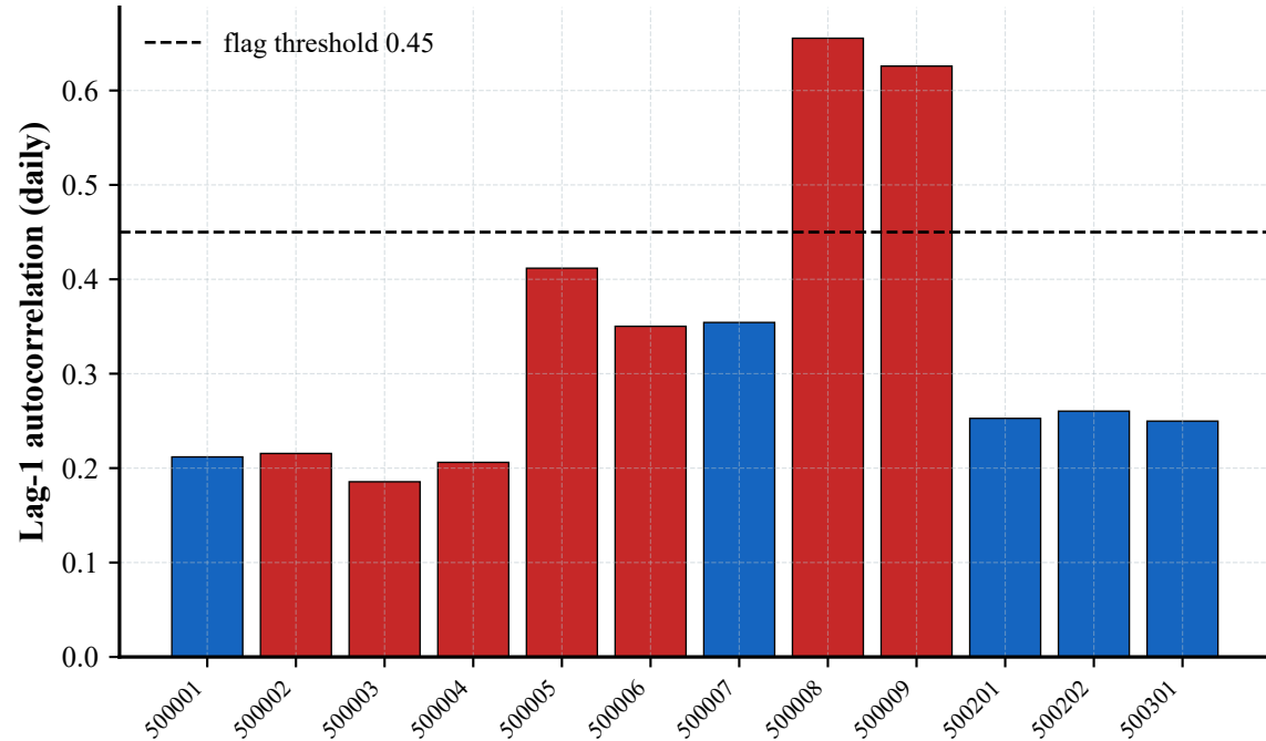
(a) Temporal smoothing diagnostic
